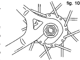
Bolt-on Rear Wheel in Dropouts
